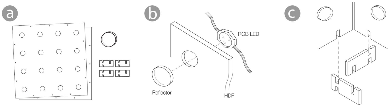
Figure 2: Construction manual for hybrid media façade toolkit: (a) laser cut wooden façade panels, acrylic reflectors and joints for assembling (b) attaching the reflectors ahead (gluing is recommended) and inserting the RGB-LED chains from back (c) assembling the modular panels with the joints.
